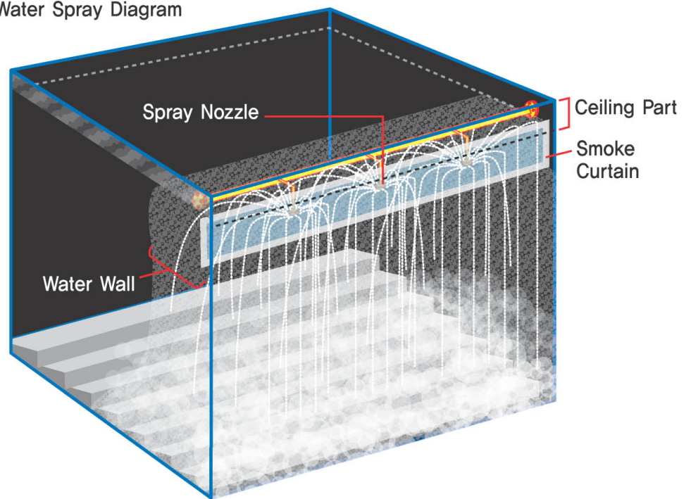
Installation in Underground Tunnel
