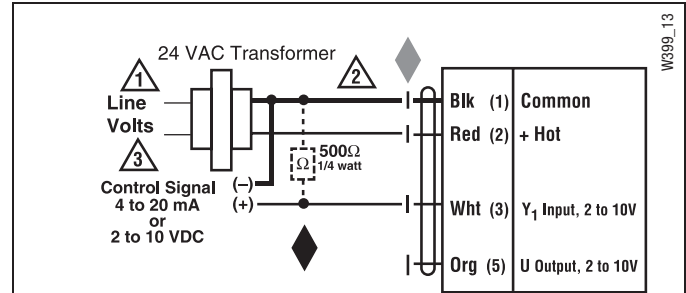
VDC/4-20 mA
