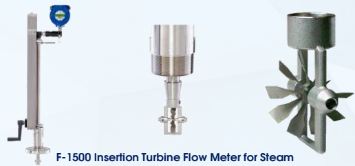
F-1500 Insertion Turbine Flow Meter for Steam
