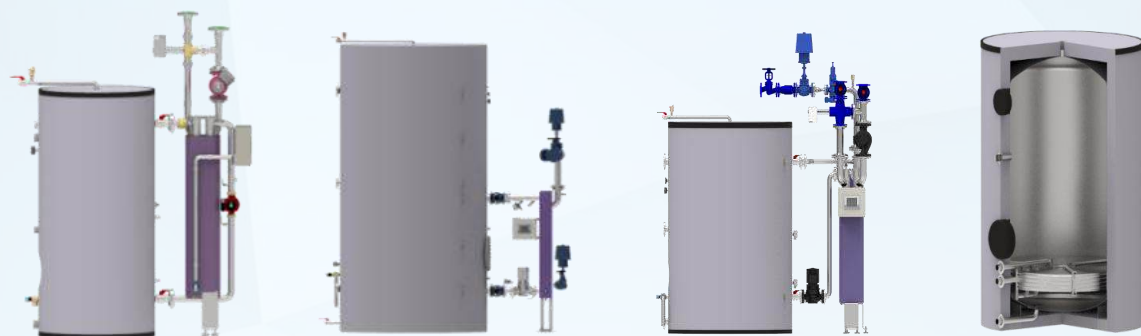
HIGH-CAPACITY WATER HEATERS WITH EXTERNAL SHELL, TUBE HEAT EXCHANGER & INTERNAL SPIRAL FLAT HEATING COIL (USE FOR WATER/STEAM BOILERS, HEAT PUMPS)
